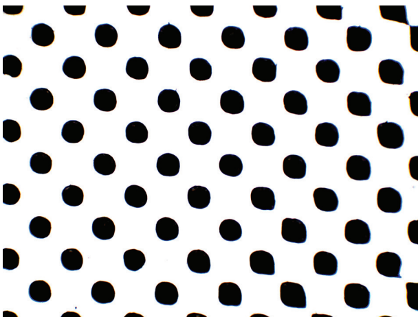
Figure 8c Letterpress halftone print at 50 lpi created using an Ives/Levy halftone screen (40x magnification in the Dmin area).
